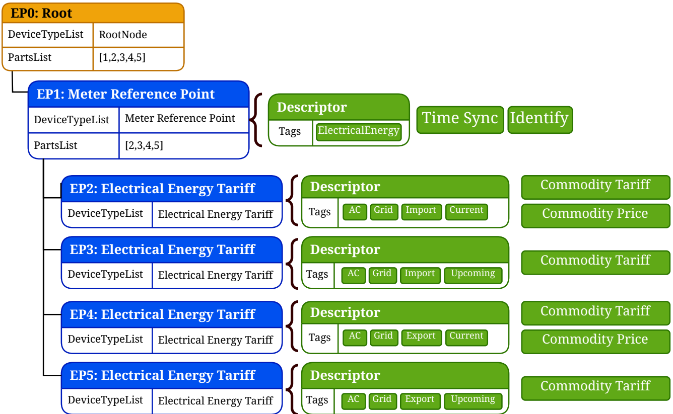
Figure 27. Example of a Meter Reference Point with an export tariff
