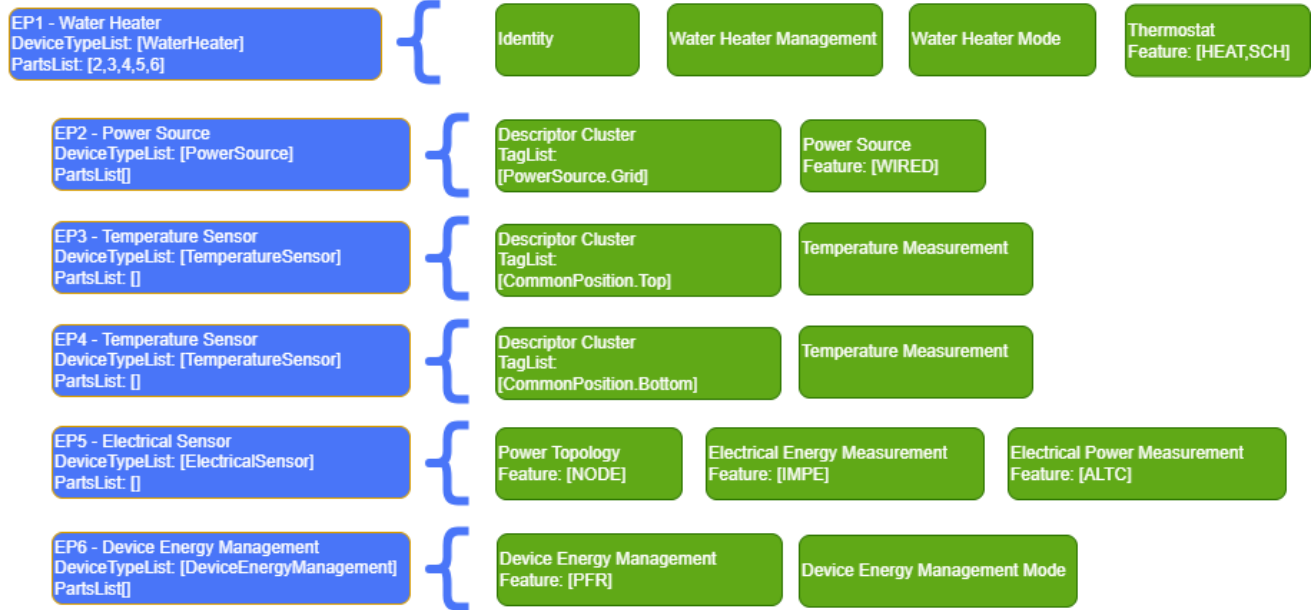
Figure 17. Example of a Water Heater
