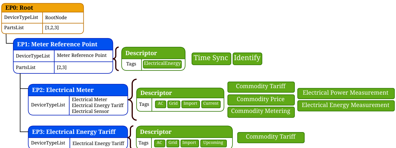
Figure 29. Example of a Meter Reference Point that supports metering
