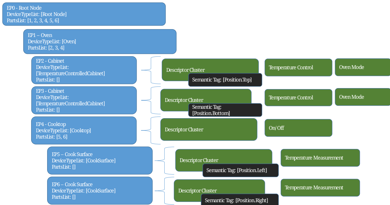
Figure 13. Example of an Oven
