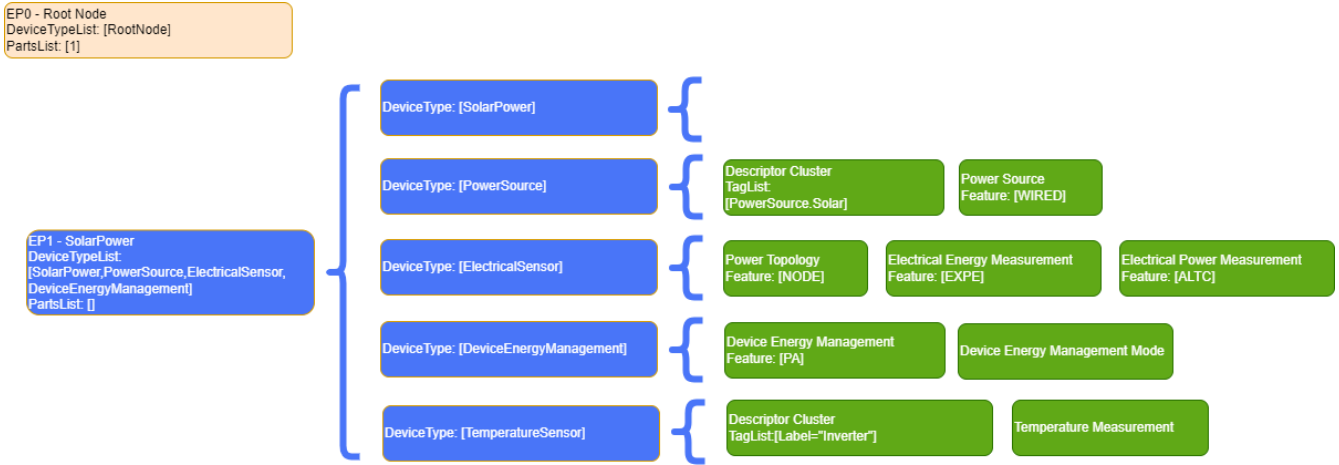
Figure 18. Example of a Solar Power device with single phase AC output
