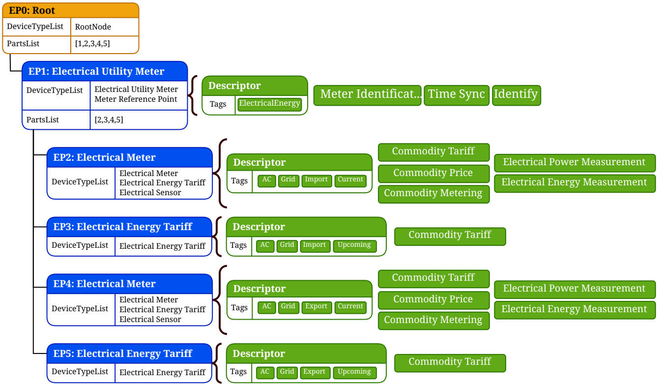
Figure 33. Example of an Electrical Utility Meter with a separate export tariff
