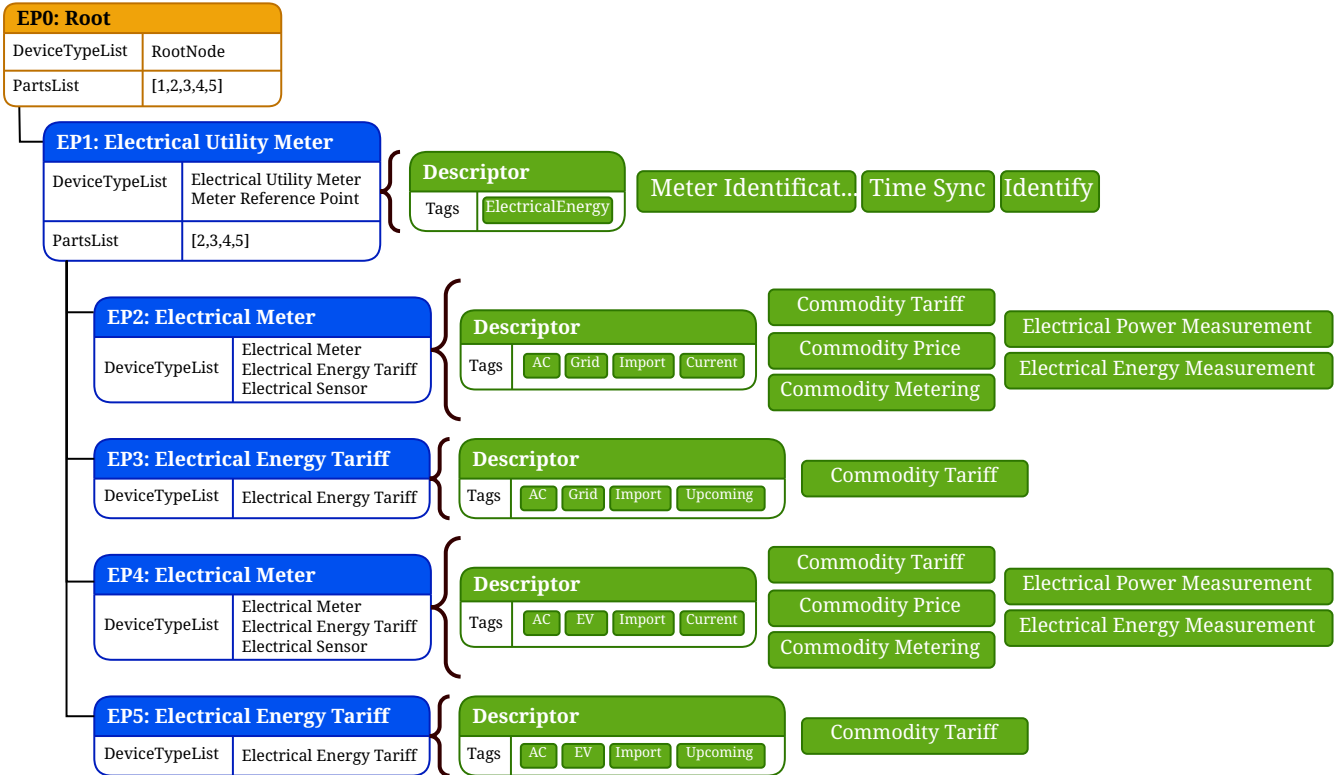
Figure 32. Example of an Electrical Utility Meter with a separate EV tariff
