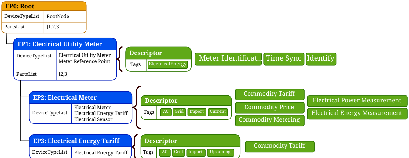
Figure 30. Example of a basic Electrical Utility Meter
