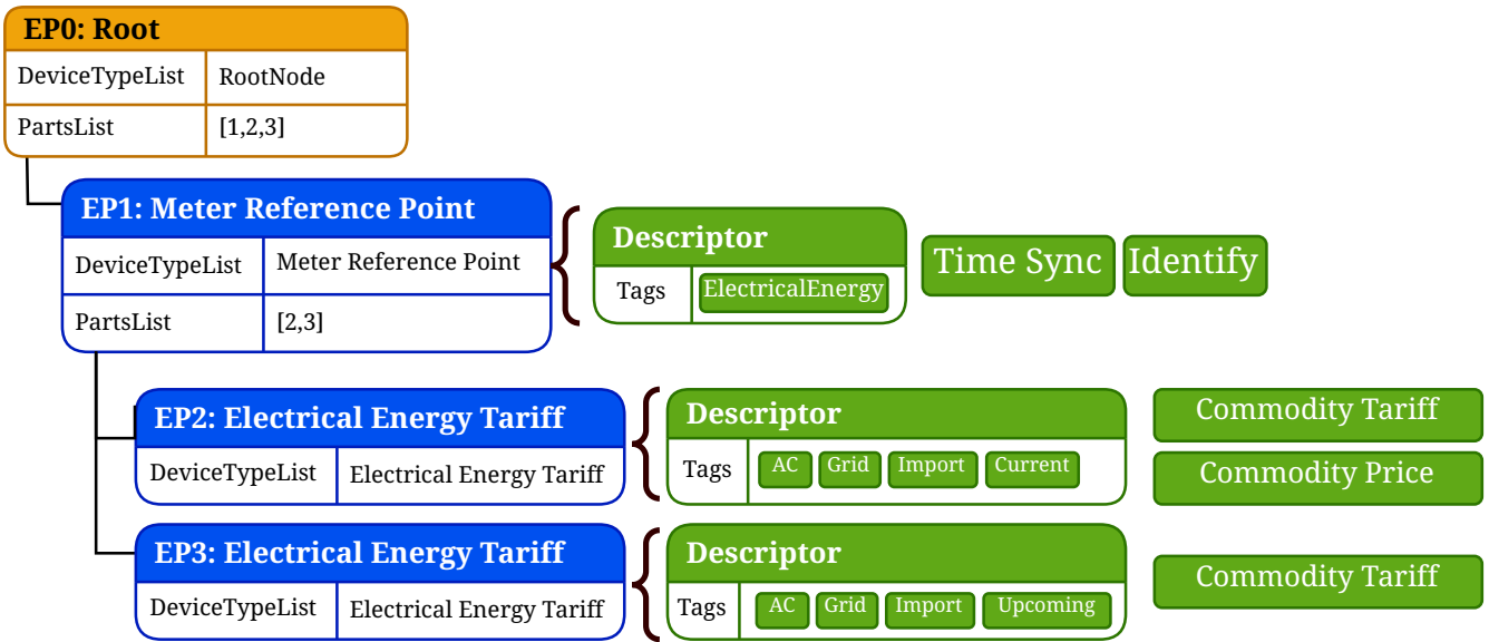
Figure 24. Example of a basic Meter Reference Point
