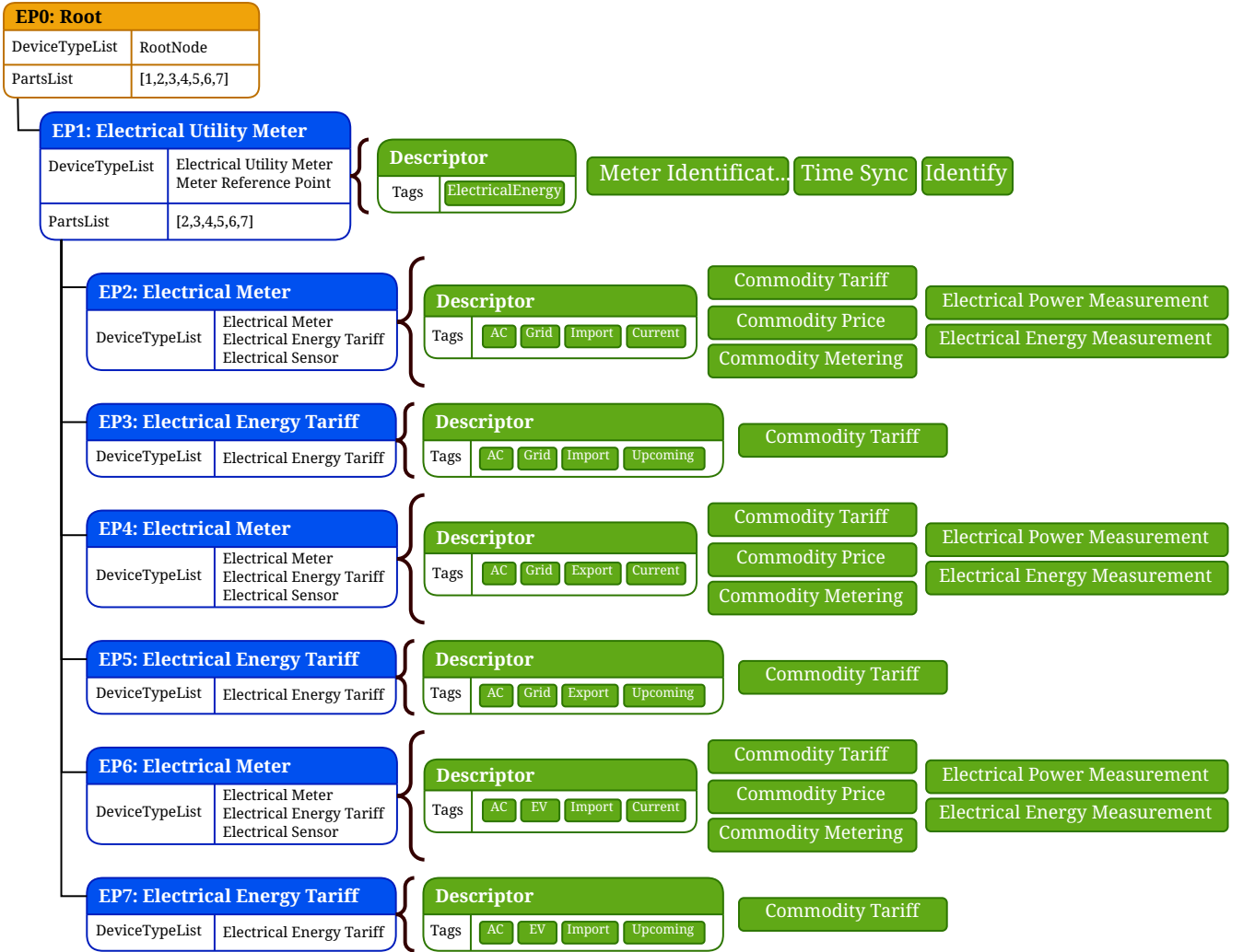
Figure 34. Example of an Electrical Utility Meter with separate export and EV tariffs
