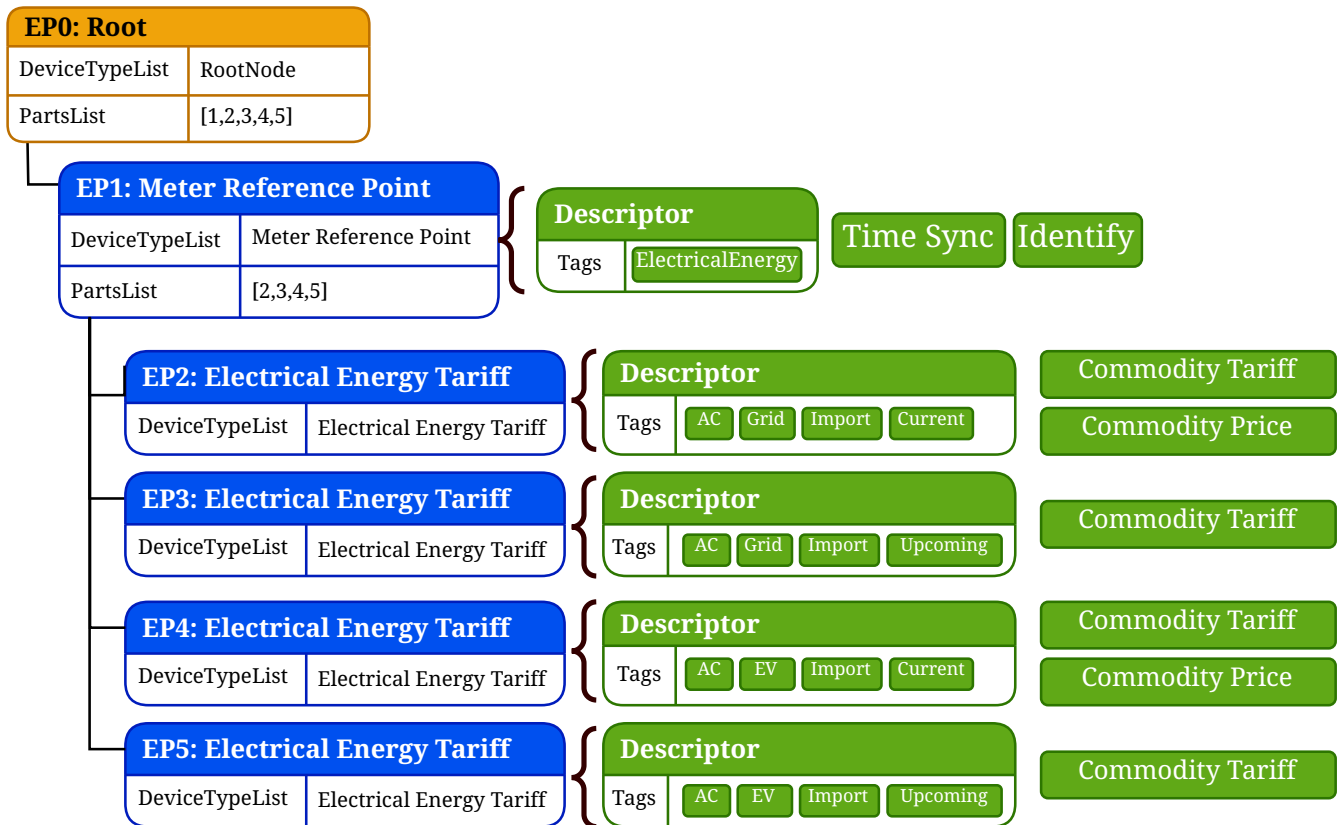
Figure 26. Example of a Meter Reference Point with a separate EV tariff
