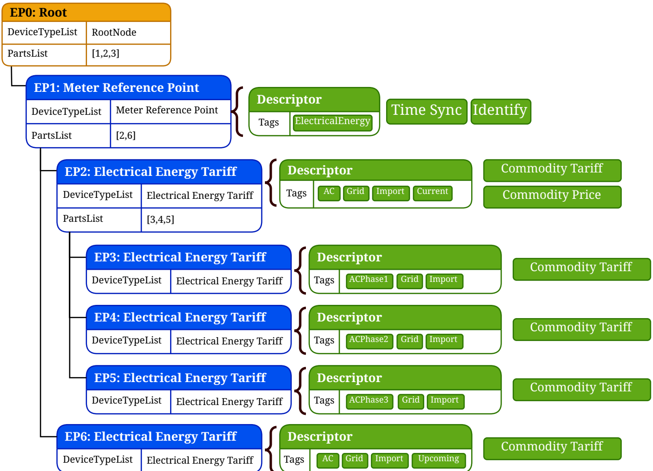
Figure 25. Example of a Meter Reference Point with multiple phases
