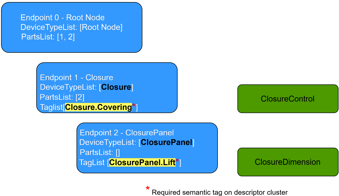
Figure 4. Example of a Closure with single panel
