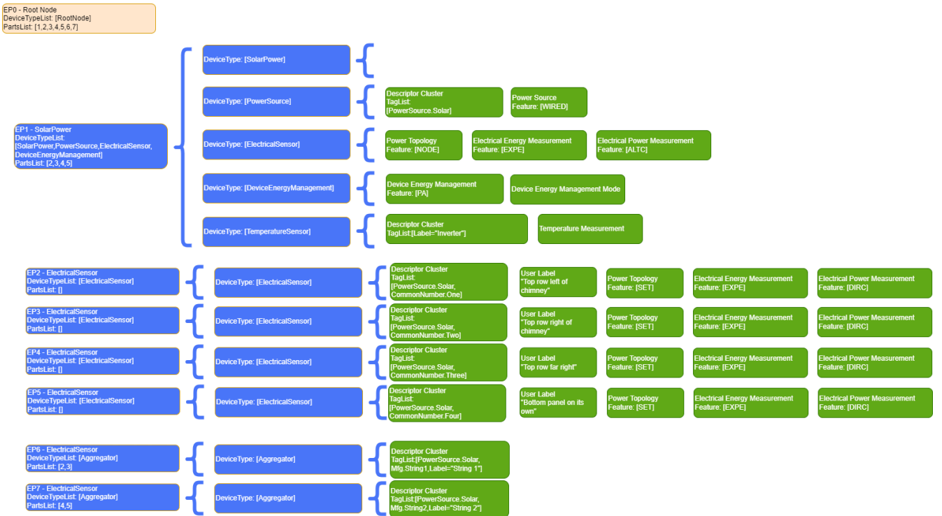
Figure 20. Example of a Solar Power device with solar panel measurements
