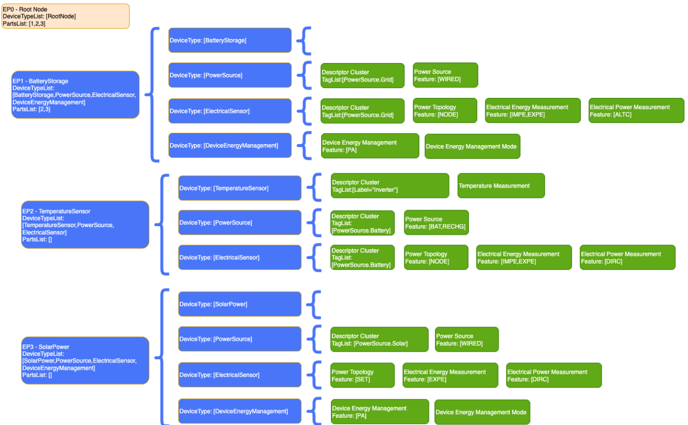
Figure 22. Example of a Battery Storage device with DC-connected Solar Power device
