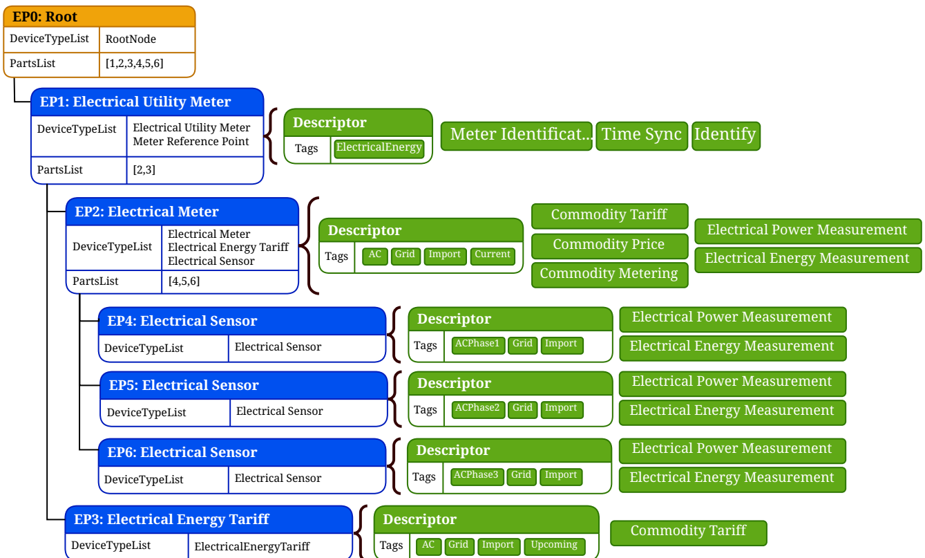
Figure 31. Example of a phased Electrical Utility Meter
