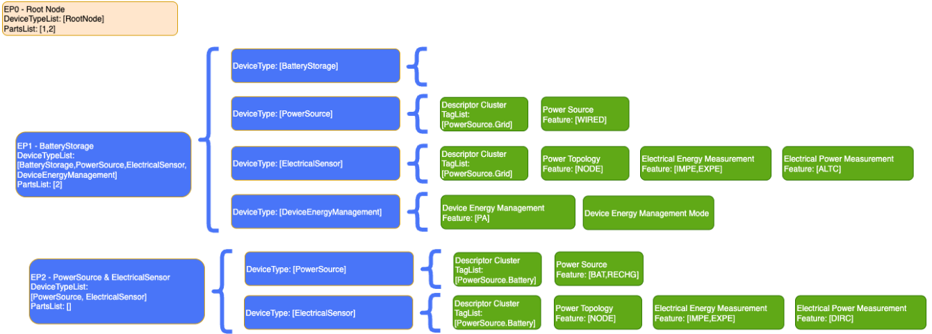
Figure 21. Example of a Battery Storage device with single phase AC output
