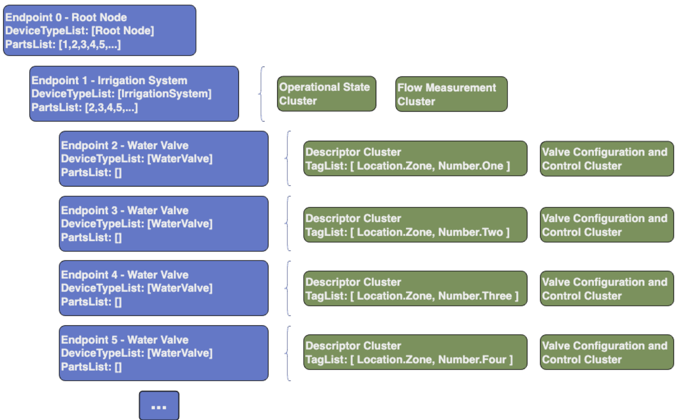
Figure 2. Example of an Irrigation System
